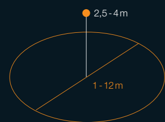
Mounting height 2,5 - 4 m Detection zone Ø 1 - 12 m / 113 m 2
