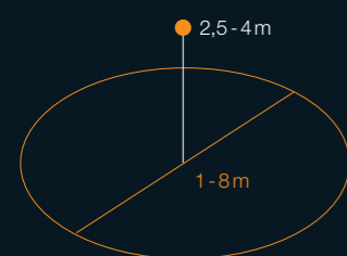
Mounting height 2.5 - 4 m Detection zone Ø 1 - 8 m / 50 m 2
